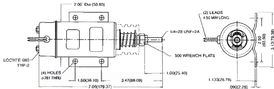
SOLENOID SHOWN ENERGIZED
