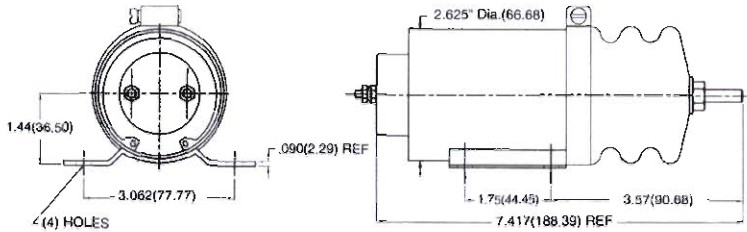
SOLENOID SHOWN DE-ENERGIZED
