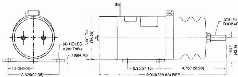
SOLENOID SHOWN DE-ENERGIZED
