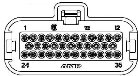
35 Pin AMPSeal 776164-1 TERMINAL 770520-1 SEALING PLUG 770678-1
