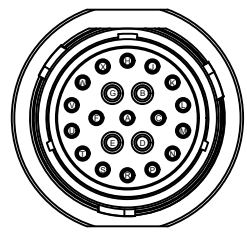
ENGINE CONNECTOR
